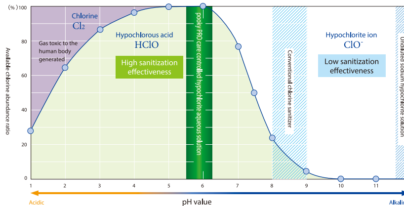
Basic Generation Principle and Abundance Ratio of Free Available Chlorine due to Change in pH
